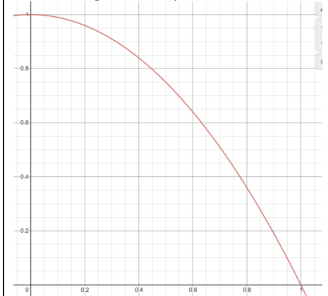
Sum Using the Midpoint Rule
